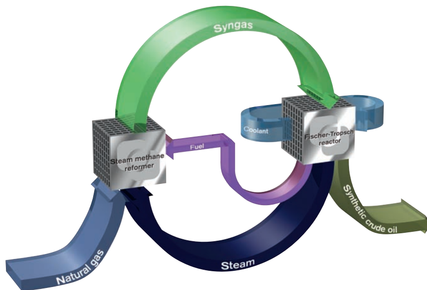
Fig. 1—Picture of the SMR/FT cycle.
