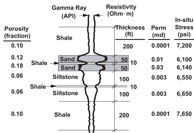
Fig. 5—Layer data required for evaluating the formation and designing the fracture treatment.
