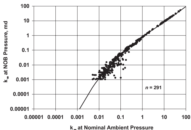
Fig. 3—Gas permeability at NOB pressure vs. gas permeability at ambient pressure for Howell No. 5 and SFE No. 2 Travis Peak cores.
