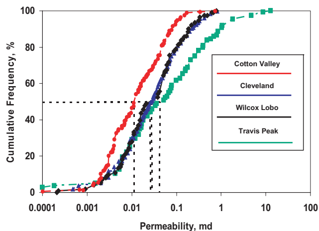
Fig. 4—Comparison of permeability distribution in four tight-sandstone gas formations in Texas using public data.
